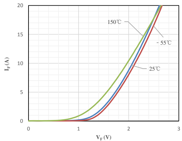
Fig 5 Body-Diode Characteristics
