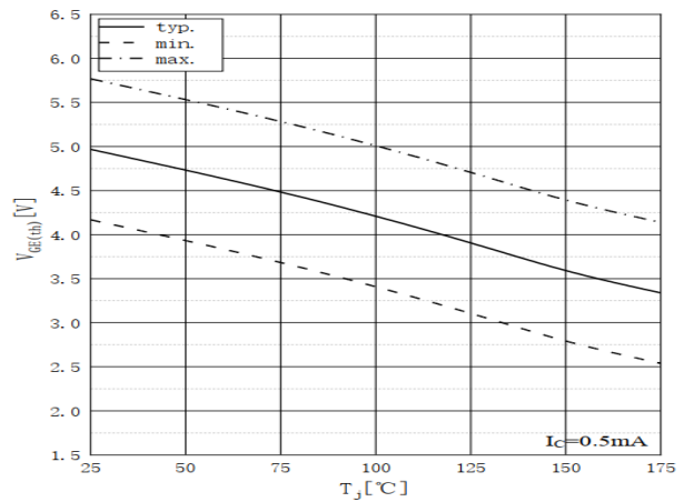
Fig 4 V_{GE(th)} vs. Junction Temperature
