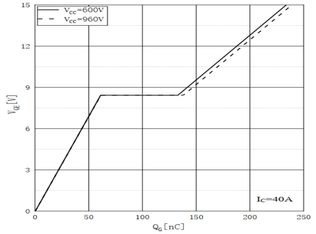
Fig 8 Gate-Charge Characteristics
