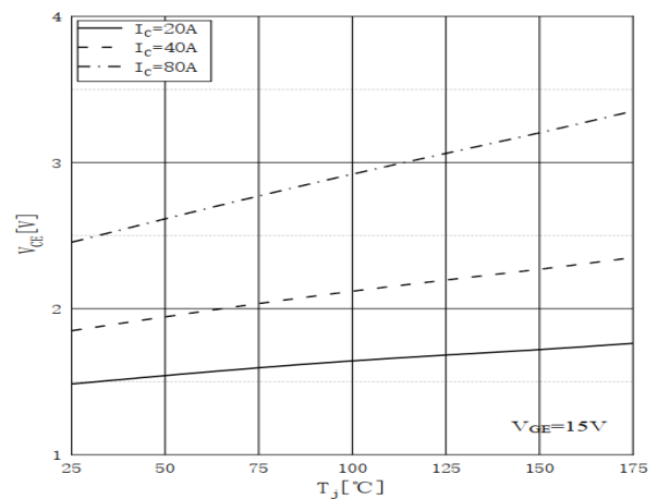
Fig 6 Collector-Emitter Saturation Voltage vs. Junction Temperature
