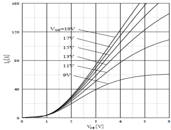
Fig 2 Saturation Voltage Characteristics ( T_j = 175^\circ\text{C} )
