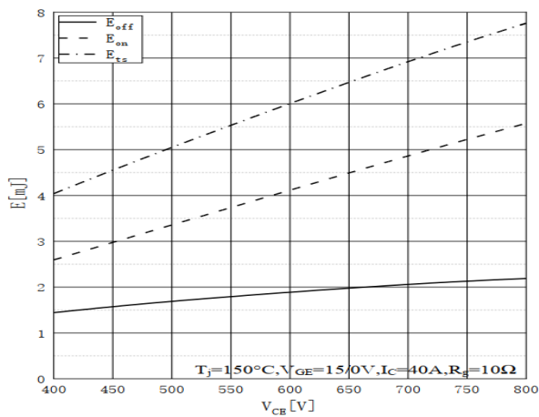
Fig 5 Switching Loss vs. Collector-Emitter Voltage
