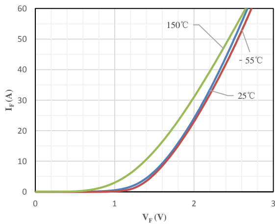
Fig 5 Body-Diode Characteristics
