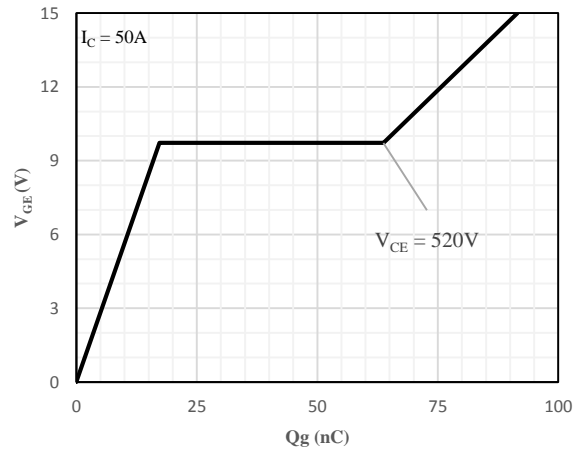
Fig 8 Gate-Charge Characteristics
