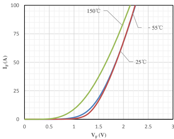
Fig 5 Body-Diode Characteristics
