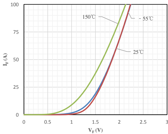
Fig 5 Body-Diode Characteristics
