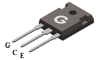
TO-247
