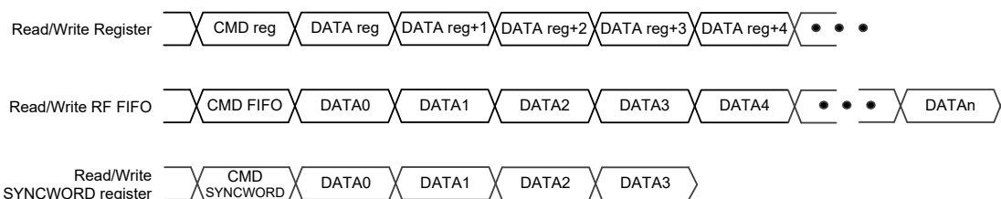
Strobe Command Followed by n-byte Data (CmdD)
