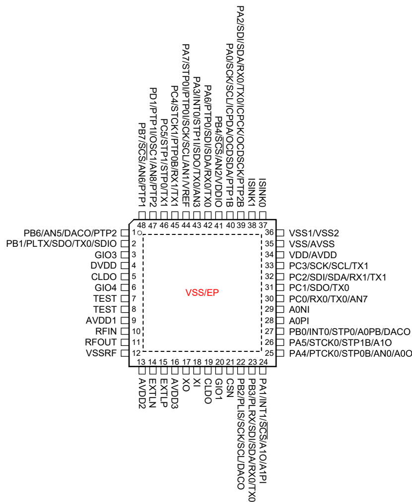
BA45F5660/BA45V5660 48 LQFP-EP
