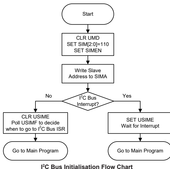
I 2 C Bus Initialisation Flow Chart
