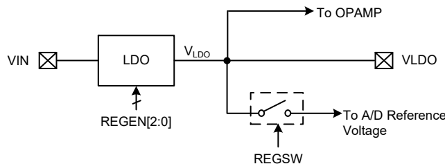
LDO Regulator
