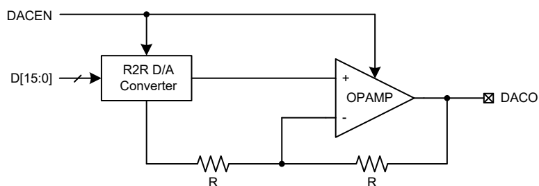
16-bit D/A Converter Block Diagram
