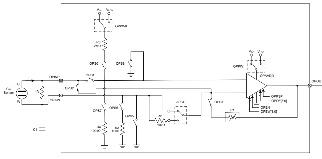
CO/Gas Detector Application Schematic
