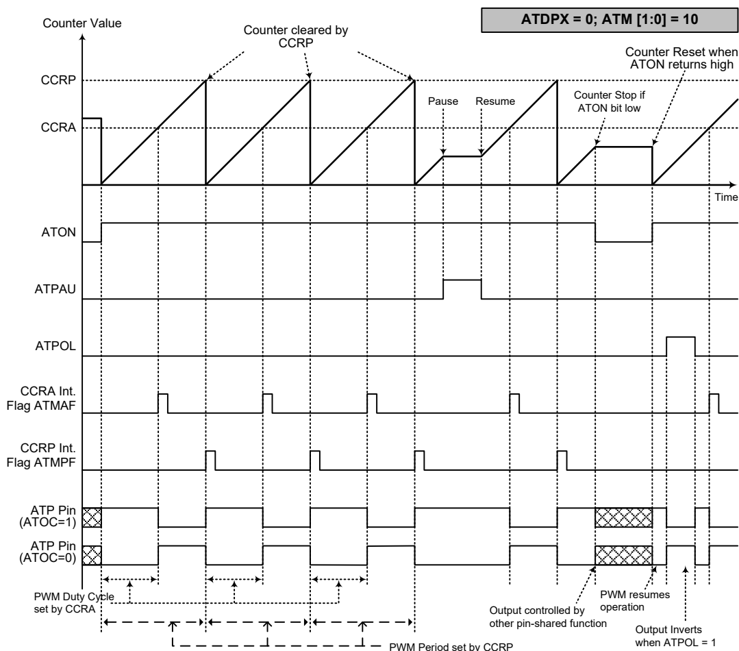
ATM Normal PWM Output Mode – ATDPX=0
