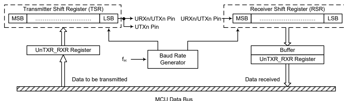
USIMn UART Data Transfer Block Diagram – UnSWM=1 (n=0~1)
