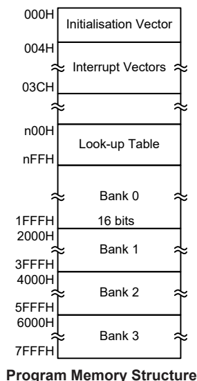
Program Memory Structure
