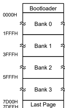
Flash Program Memory Structure including Bootloader
