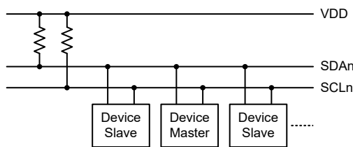
USIMn I 2 C Master Slave Bus Connection
