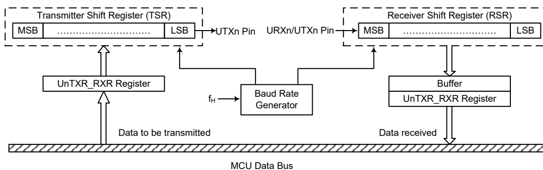
USIMn UART Data Transfer Block Diagram – UnSWM=0 (n=0~1)
