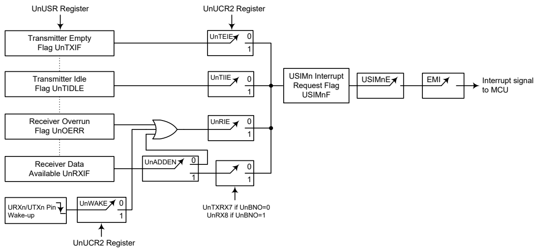
USIMn UART Interrupt Structure
