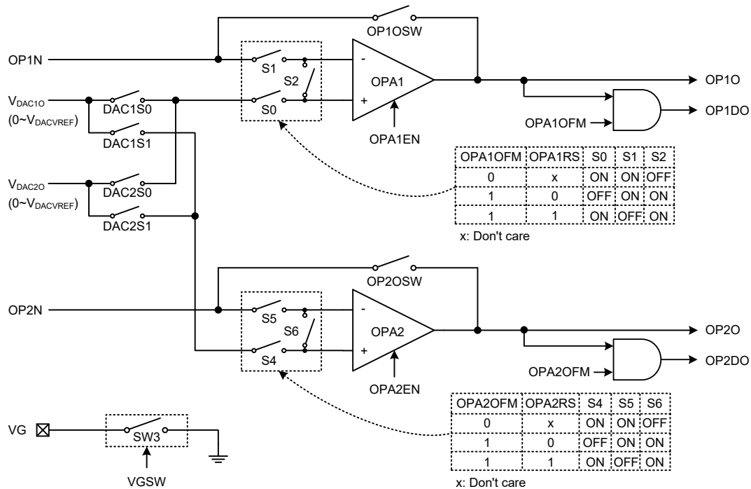
Operational Amplifier Structure
