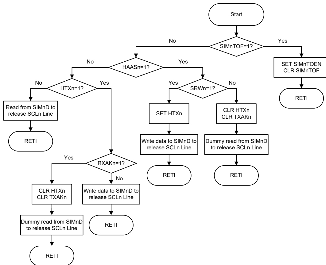
USIMn I²C Bus ISR Flow Chart
