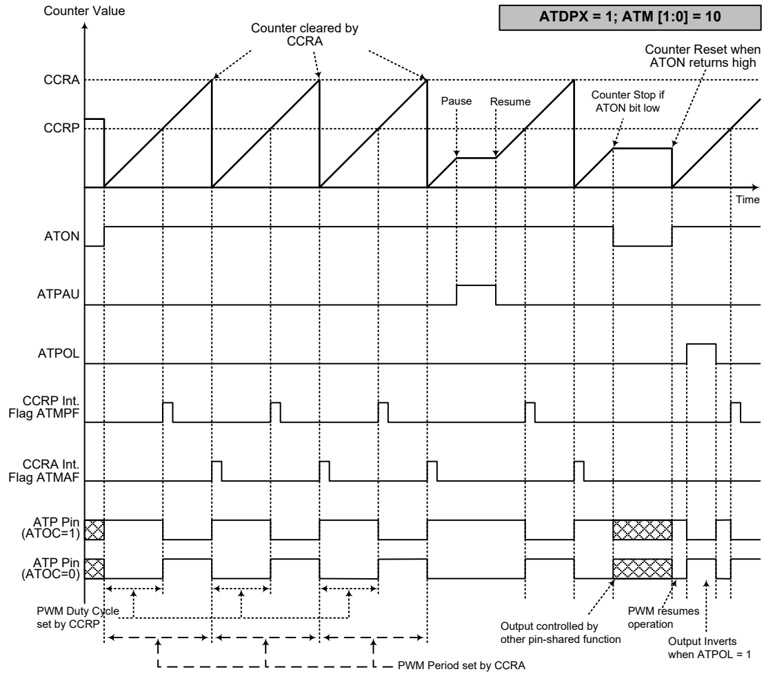
ATM Normal PWM Output Mode – ATDPX=1
