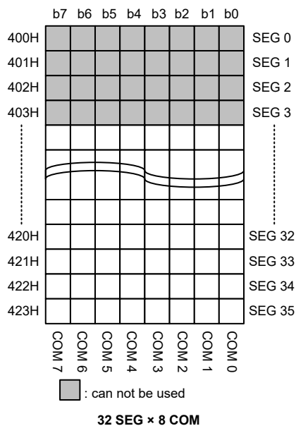
LCD Memory Map
