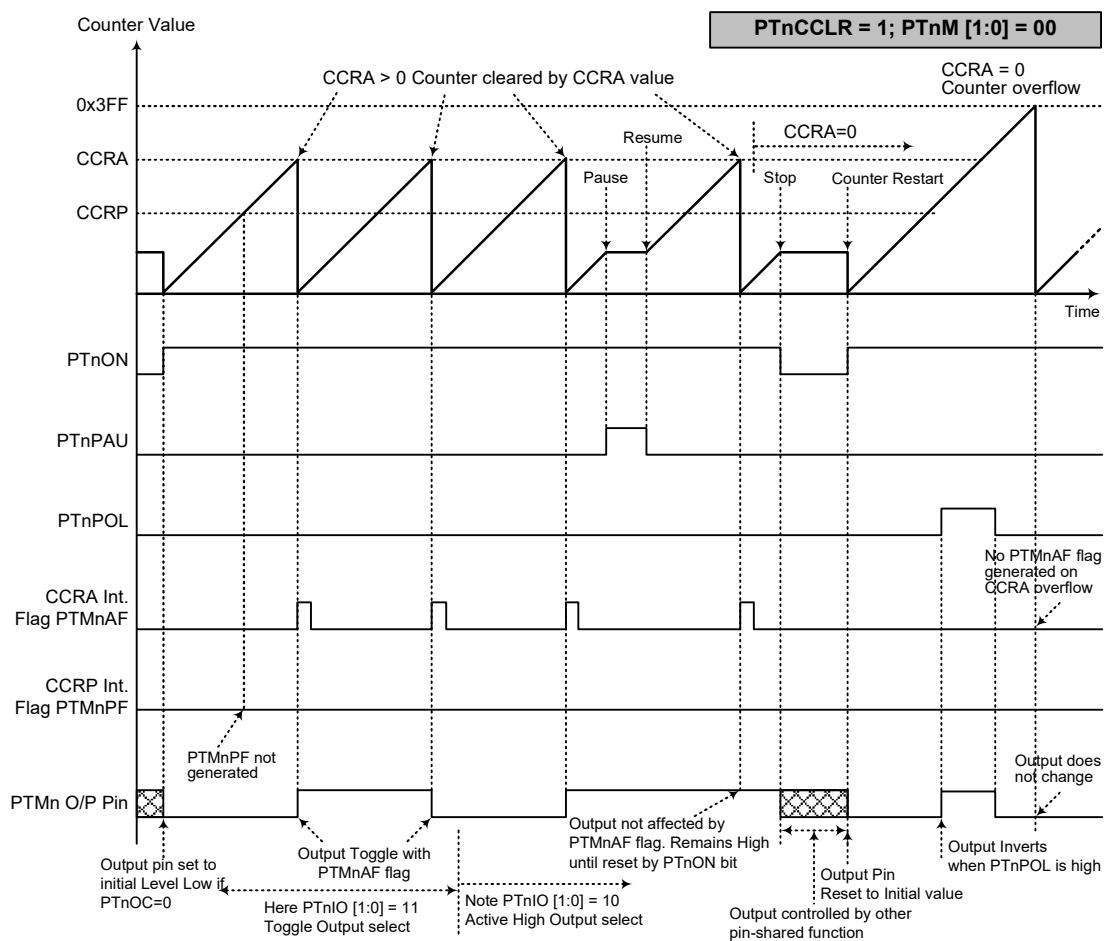
Compare Match Output Mode – PTnCCLR=1 (n=0~1)
