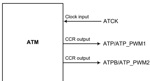
ATM Function Pin Block Diagram
