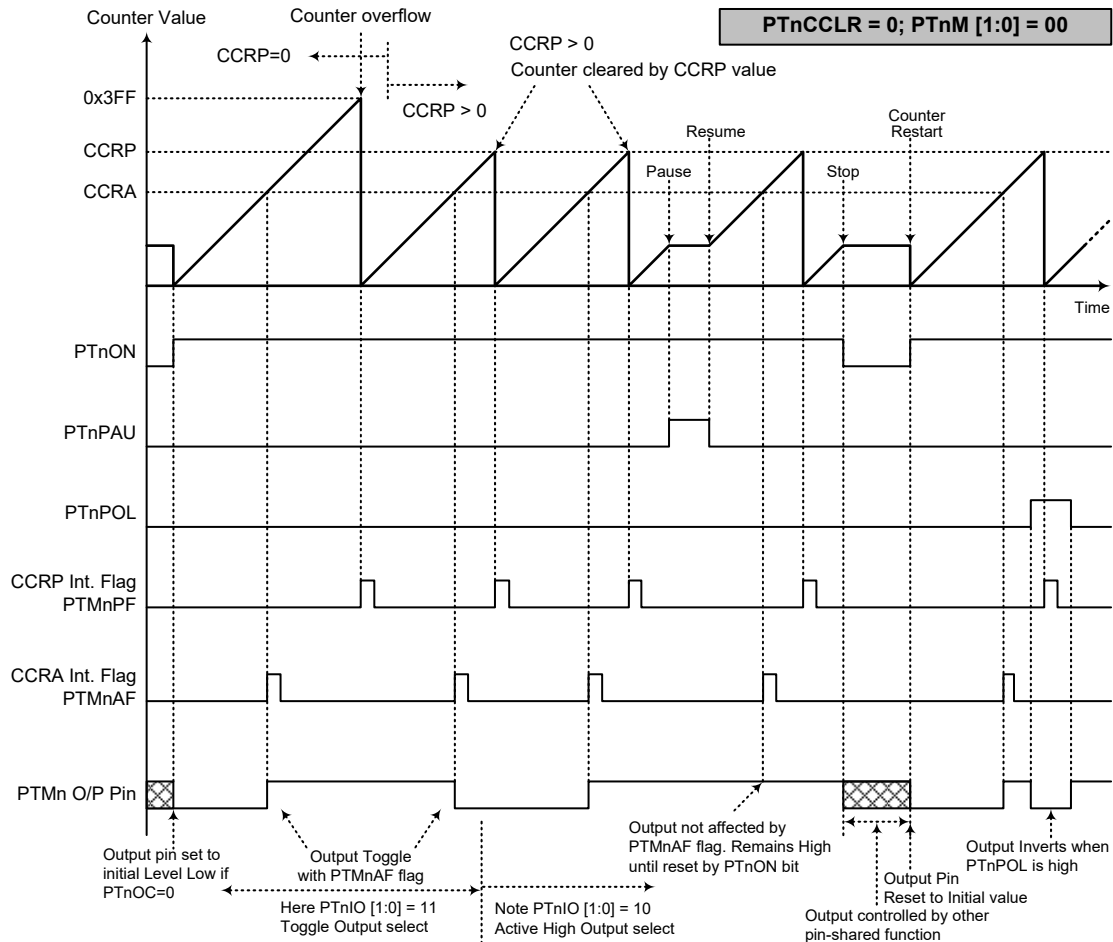
Compare Match Output Mode – PTnCCR=0 (n=0~1)
