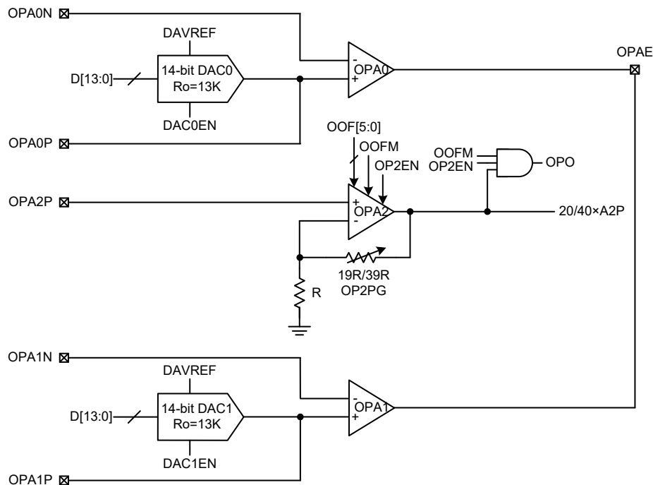
Battery Charge Module Structure
