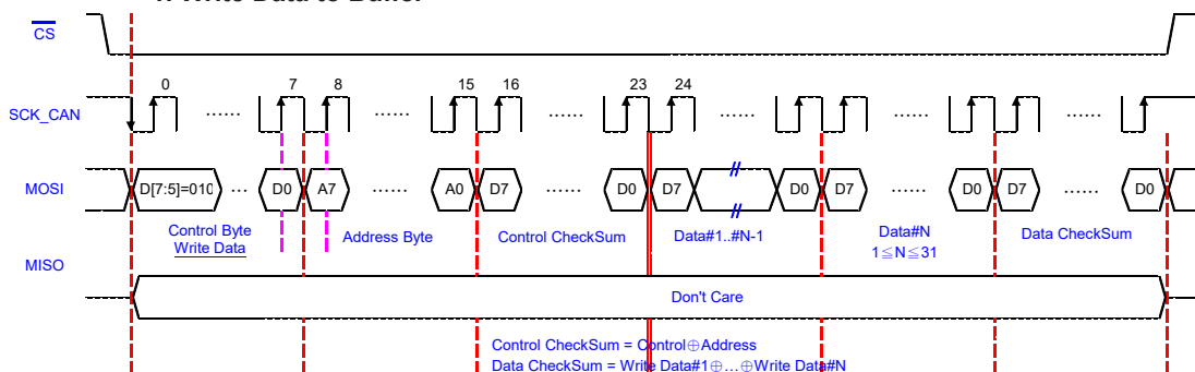
Write Data to Buffer Timing Diagram
