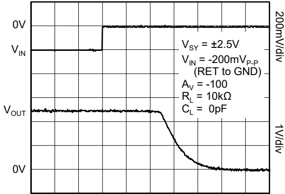
Time (20 \mu s/div)
