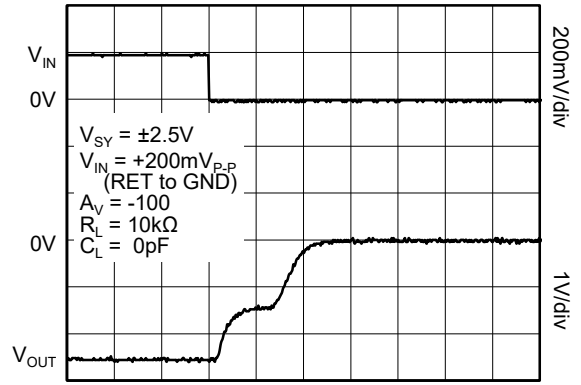
Time (50 \mu s/div)
