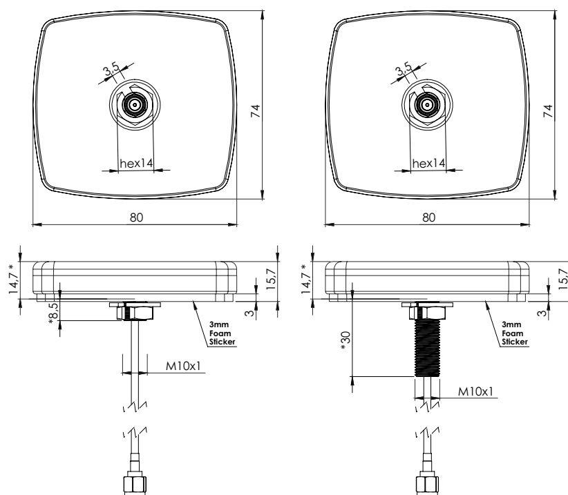
2J6015B-868-TH8,5 8,5 mm Thread
