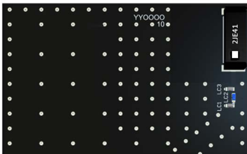
3D View of matching components and recommended values (LC1=3.9 pF, LC2=10 pF, LC3=DNP)
