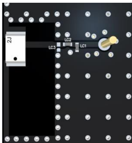
3D View of matching components and recommended values (LC1=11.0pF \pm 5\% , LC2=2.4pF \pm 0.05\text{pF} , LC3=OPEN)
