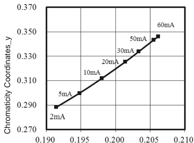
Chromaticity Coordinates vs. Forward Current (Ta=25°C)
