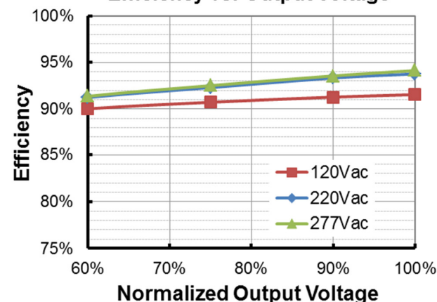
EUD-600S12ADV(I o =10000mA) Efficiency vs. Output Voltage
