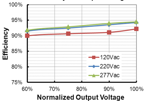
EUD-600S980DV(I o =7840mA) Efficiency vs. Output Voltage
