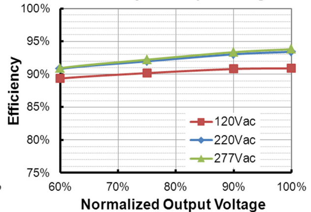
EUD-600S740DV(I o =7400mA) Efficiency vs. Output Voltage
