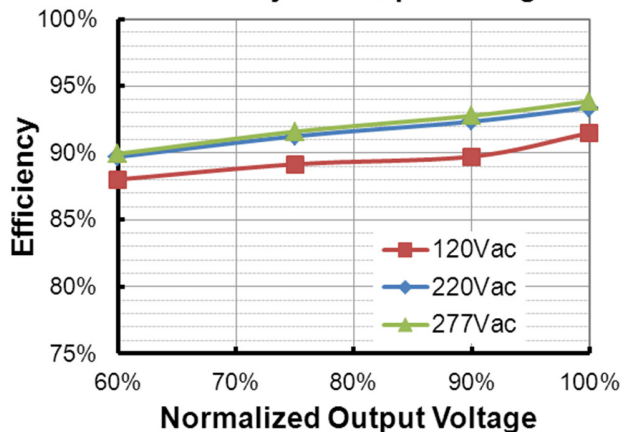
EUD-600S980DV(I o =9800mA) Efficiency vs. Output Voltage
