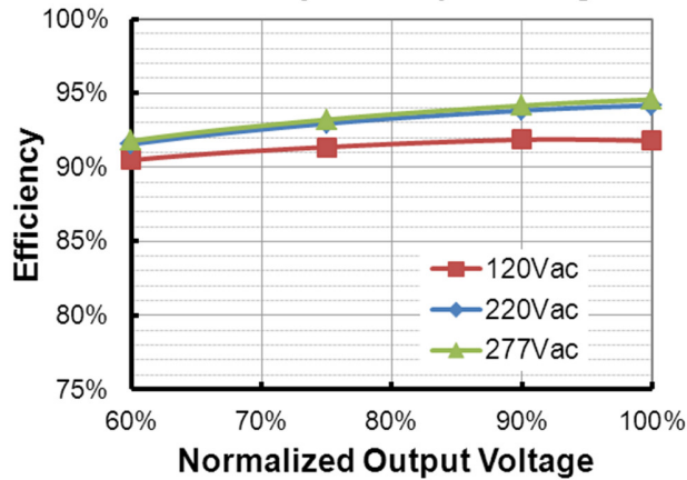
EUD-600S740DV(I o =5920mA) Efficiency vs. Output Voltage
