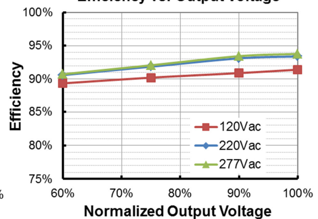
EUD-600S12ADV(I o =12500mA) Efficiency vs. Output Voltage
