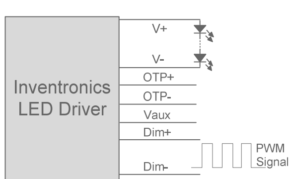
Implementation 3: Negative logic
