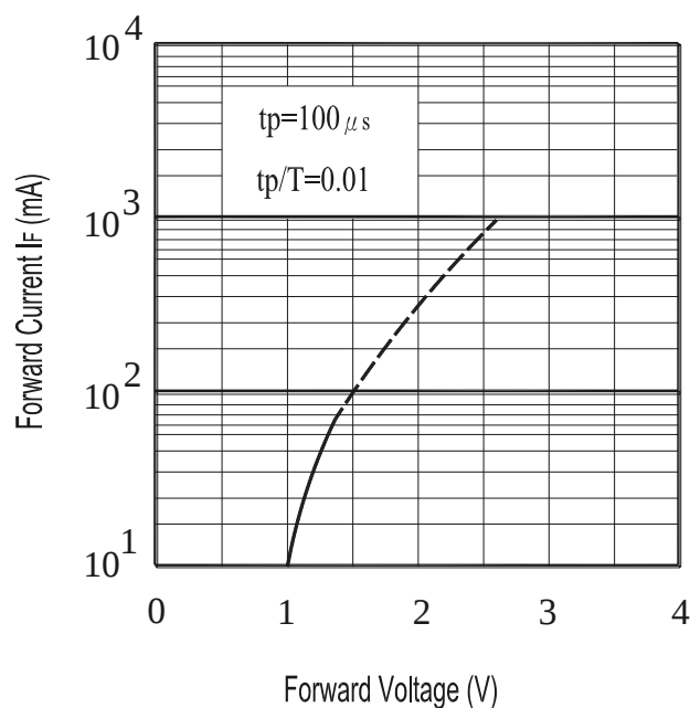
Fig.4 Forward Current
